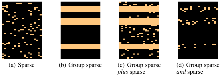
Figure 1: A comparison of different sparsity patterns. (a) shows a standard sparsity pattern. An example of group sparse patterns promoted by Glasso [21] is shown in (b). In (c), we show the patterns considered in [7]. Finally, in (d), we show the patterns we are interested in this paper.
