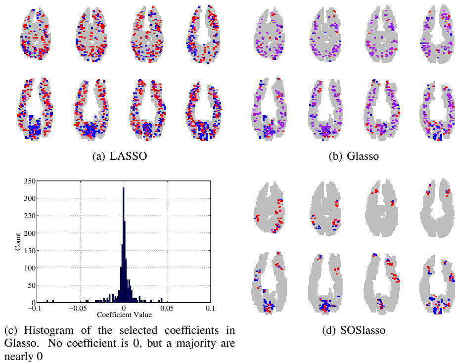
Figure 4: Per-slice result of the aggregated sparsity patterns across 6 subjects.
